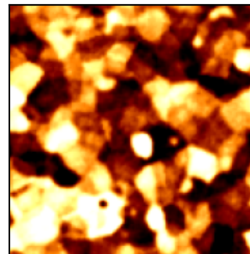
same model: auto Rq=3.56, C=88
