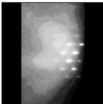
auto RHEED | Cq=75
