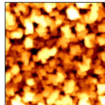
measured AFM Rq=3.05
