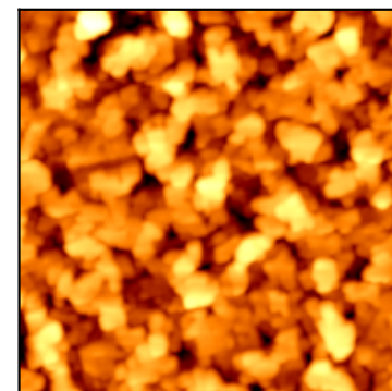
measured AFM Rq=2.56
