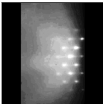
auto RHEED | Cq=57
