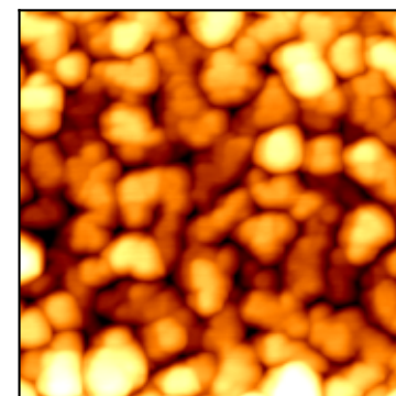
measured AFM Rq=3.18
