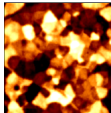
same model: auto Rq=3.05, C=90
