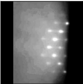
6063 human RHEED
