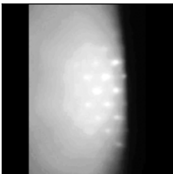
auto RHEED | Cq=70
