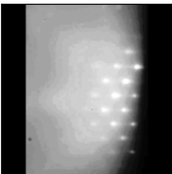
6057 human RHEED
