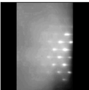
6090 human RHEED
