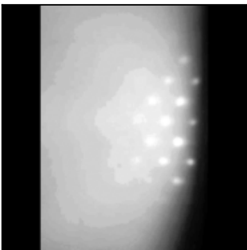
6080 human RHEED
