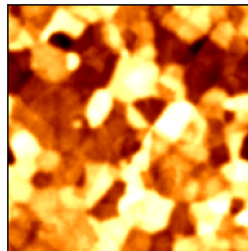
same model: auto Rq=3.21, C=97
