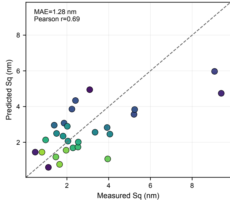
Sq: strict 27-fold automatic-input LOO
