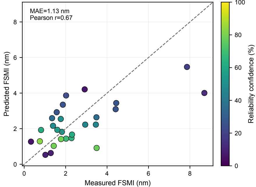
FSMI: strict 27-fold automatic-input LOO
