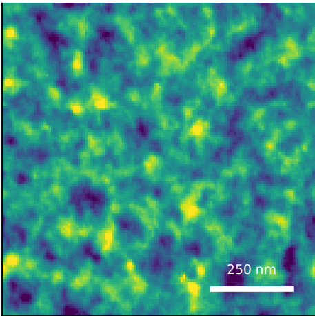
generated AFM predicted Sq=0.83 nm; FSMI=0.53 nm C=32/100
