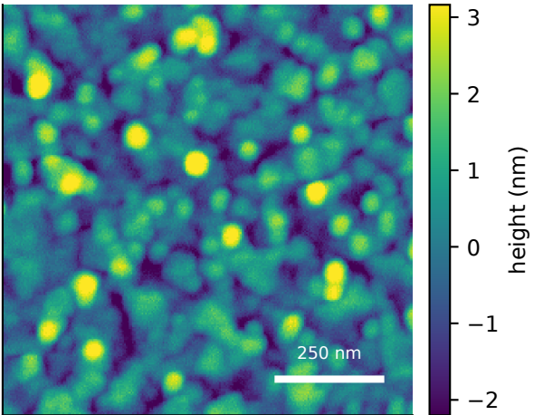
measured AFM displayed scan Sq=1.40 nm sample median Sq=1.39 ± 0.37 nm (IQR)
