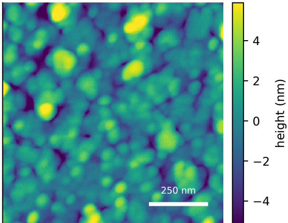
measured AFM displayed scan Sq=2.05 nm sample median Sq=2.05 ± 0.06 nm (IQR)
