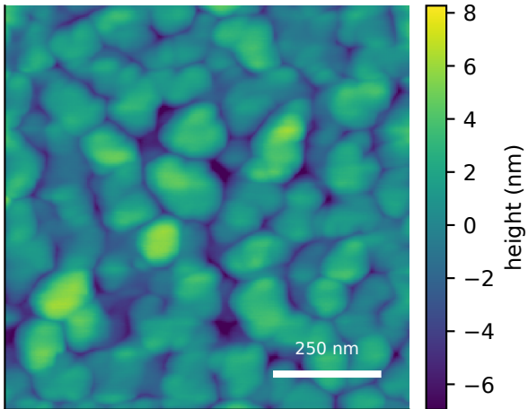
measured AFM displayed scan Sq=2.29 nm sample median Sq=2.29 ± 0.15 nm (IQR)
