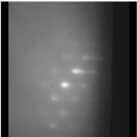
N6389 RHEED key frame
