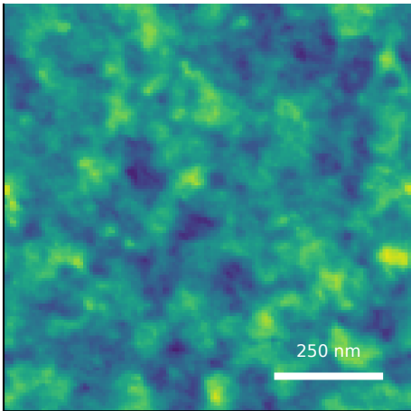
generated AFM predicted Sq=2.88 nm; FSMI=2.55 nm C=93/100
