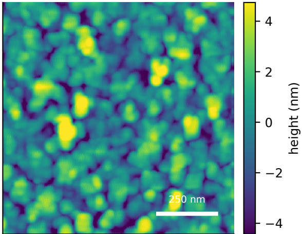
measured AFM displayed scan Sq=2.02 nm sample median Sq=2.02 ± 0.13 nm (IQR)
