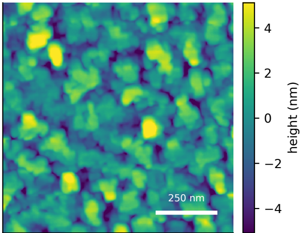
measured AFM displayed scan Sq=2.18 nm sample median Sq=2.24 ± 0.18 nm (IQR)
