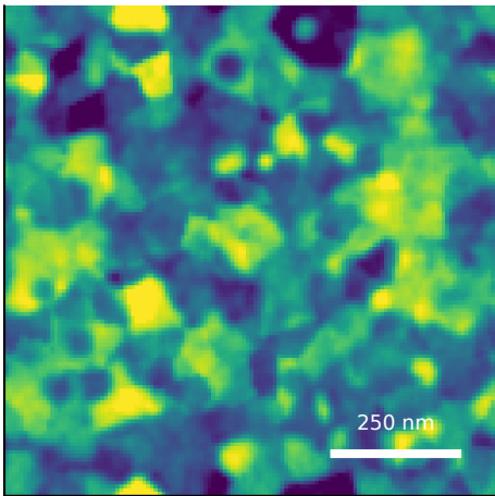
generated AFM predicted Sq=4.71 nm; FSMI=3.35 nm C=21/100
