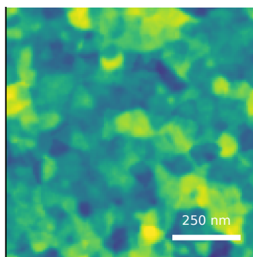
M17b topology-conditioned sparse peaks sample median S_q=3.93 \pm 0.28 nm (IQR) measured AFM displayed scan S_q=4.21 nm
