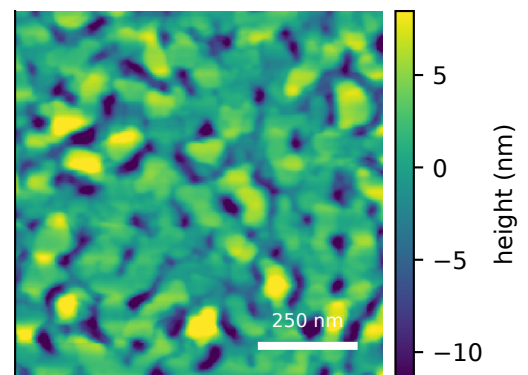
M17b topology-conditioned sparse peaks sample median S_q=3.93 \pm 0.28 nm (IQR) measured AFM displayed scan S_q=4.21 nm
