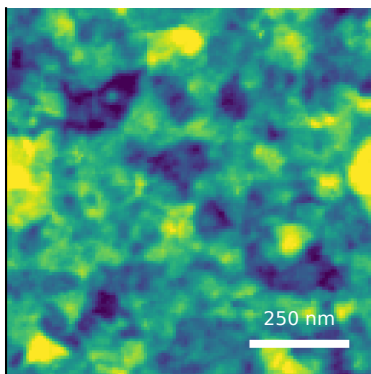
M10 baseline predicted S_q=2.73 nm
