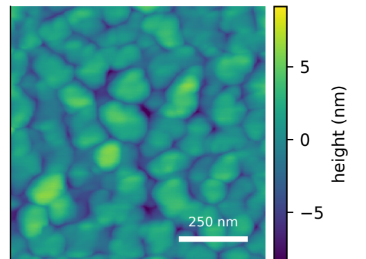
M17b topology-conditioned sparse peaks sample median S_q=2.24 \pm 0.18 nm (IQR) measured AFM displayed scan S_q=2.18 nm
