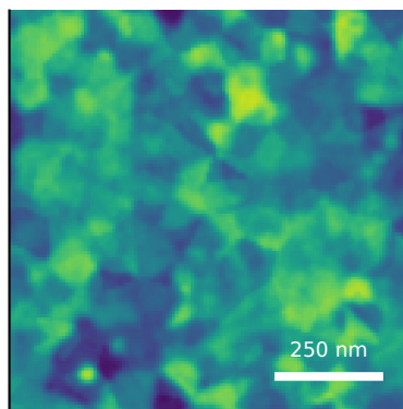
M17b topology-conditioned sparse peaks sample median S_q=9.39 \pm 0.21 nm (IQR) measured AFM displayed scan S_q=9.39 nm
