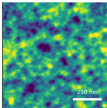
M17b topology-conditioned sparse peaks sample median S_q=0.48 \pm 0.09 nm (IQR) measured AFM displayed scan S_q=0.57 nm
