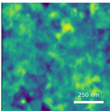
M10 baseline predicted S_q=5.52 nm
