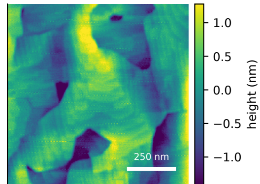
M17b topology-conditioned sparse peaks sample median S_q=0.48 \pm 0.09 nm (IQR) measured AFM displayed scan S_q=0.57 nm
