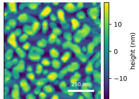
M17b topology-conditioned sparse peaks sample median S_q=9.39 \pm 0.21 nm (IQR) measured AFM displayed scan S_q=9.39 nm
