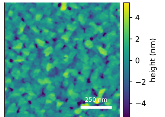
M17b topology-conditioned sparse peaks sample median S_q=1.50 \pm 0.18 nm (IQR) measured AFM displayed scan S_q=1.56 nm
