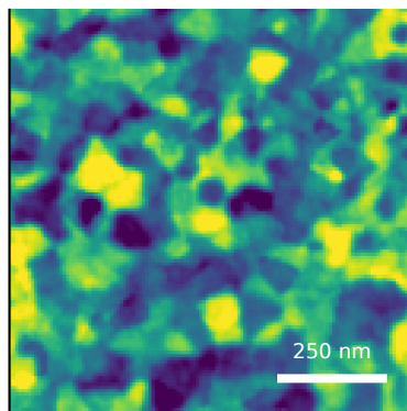
M17b topology-conditioned sparse peaks sample median S_q=1.50 \pm 0.18 nm (IQR) measured AFM displayed scan S_q=1.56 nm
