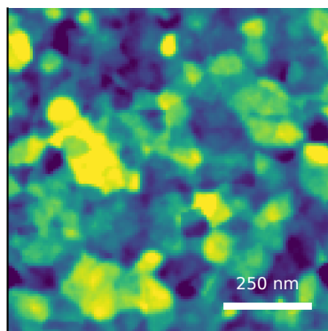
M17b topology-conditioned sparse peaks sample median S_q=2.24 \pm 0.18 nm (IQR) measured AFM displayed scan S_q=2.18 nm
