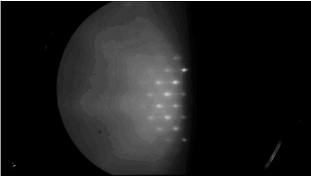
6062 RHEED key frame
