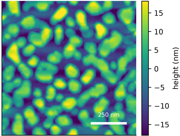
measured AFM displayed scan Sq=3.18 nm sample median Sq=3.09 ± 0.25 nm (IQR)
