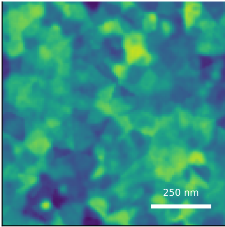
generated AFM predicted Sq=6.17 nm; FSMI=4.21 nm C=14/100
