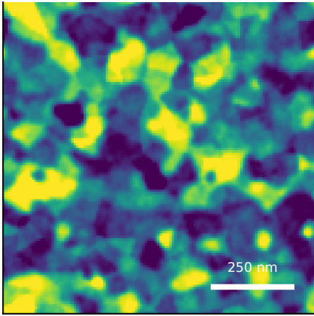
generated AFM predicted Sq=5.13 nm; FSMI=3.87 nm C=36/100
