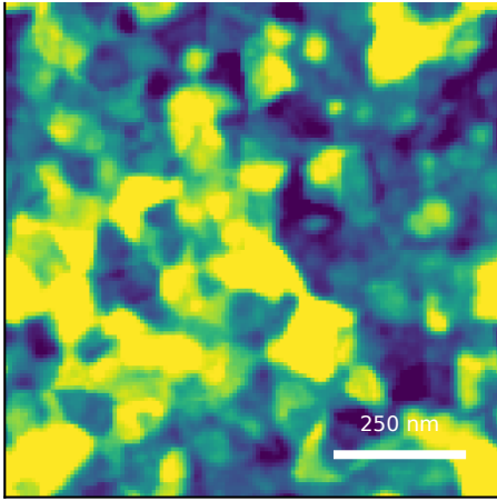
generated AFM predicted Sq=1.01 nm; FSMI=0.92 nm C=100/100
