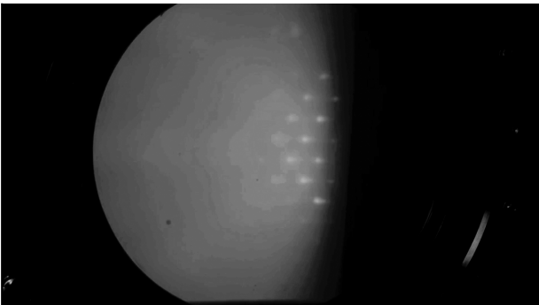
6090 RHEED key frame
