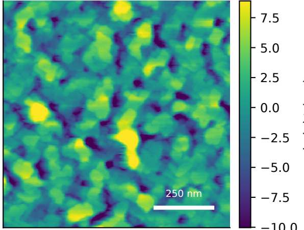
measured AFM displayed scan Sq=2.41 nm sample median Sq=2.41 ± 0.06 nm (IQR)
