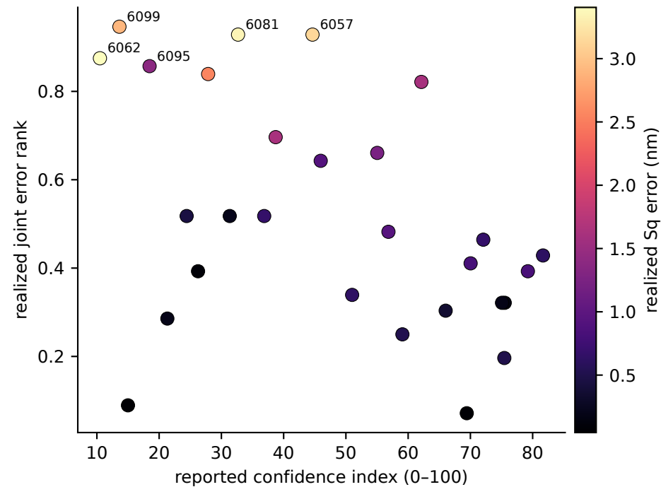
Confidence is error-related: Spearman \rho=-0.46 , p=0.015
