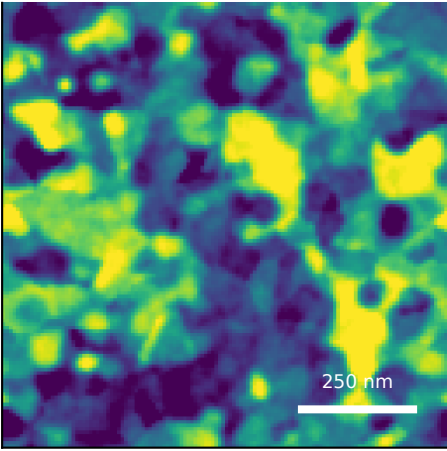
generated AFM predicted Sq=0.83 nm; FSMI=0.70 nm C=45/100
