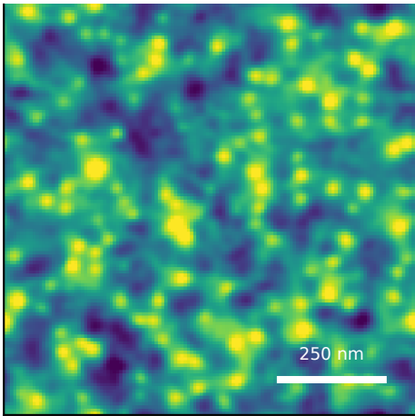
generated AFM predicted Sq=0.95 nm; FSMI=1.61 nm C=76/100
