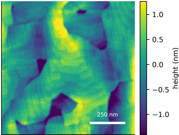
measured AFM displayed scan Sq=0.80 nm sample median Sq=0.80 ± 0.07 nm (IQR)
