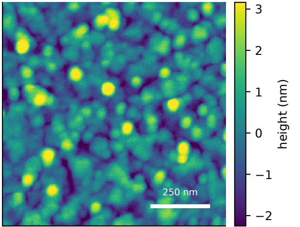
measured AFM displayed scan Sq=1.12 nm sample median Sq=1.11 ± 0.07 nm (IQR)
