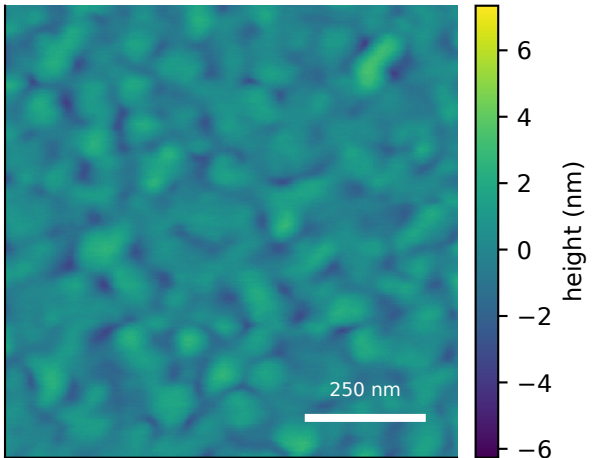
measured AFM displayed scan Sq=0.98 nm sample median Sq=0.98 ± 0.09 nm (IQR)
