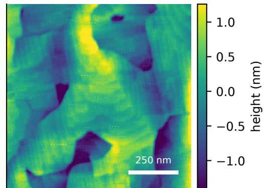
measured AFM displayed scan S_q=1.56 nm sample median S_q=1.50 \pm 0.18 nm (IQR)
