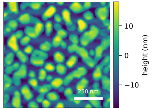
measured AFM displayed scan S_q=9.39 nm sample median S_q=9.39 \pm 0.21 nm (IQR)
