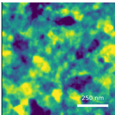
M10 baseline predicted S_q=2.72 nm
