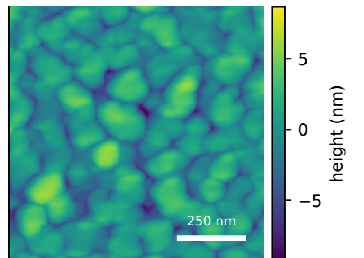
measured AFM displayed scan S_q=2.00 nm sample median S_q=3.35 \pm 3.02 nm (IQR)
