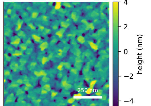
measured AFM displayed scan S_q=2.18 nm sample median S_q=2.24 \pm 0.18 nm (IQR)
