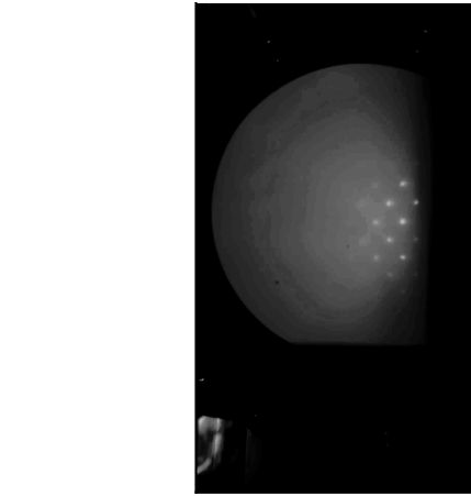
6099 RHEED key frame
