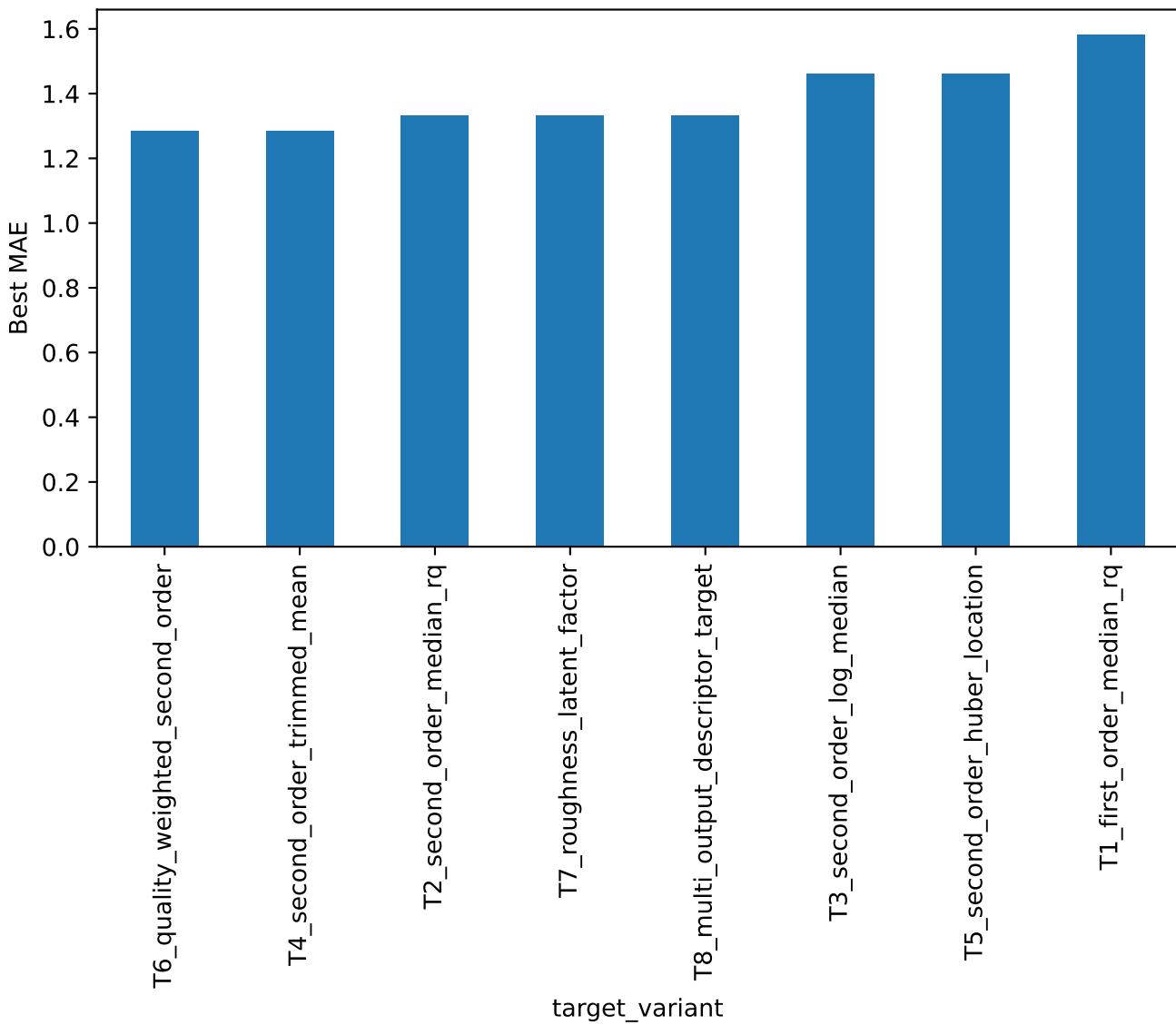
Prediction ablation
