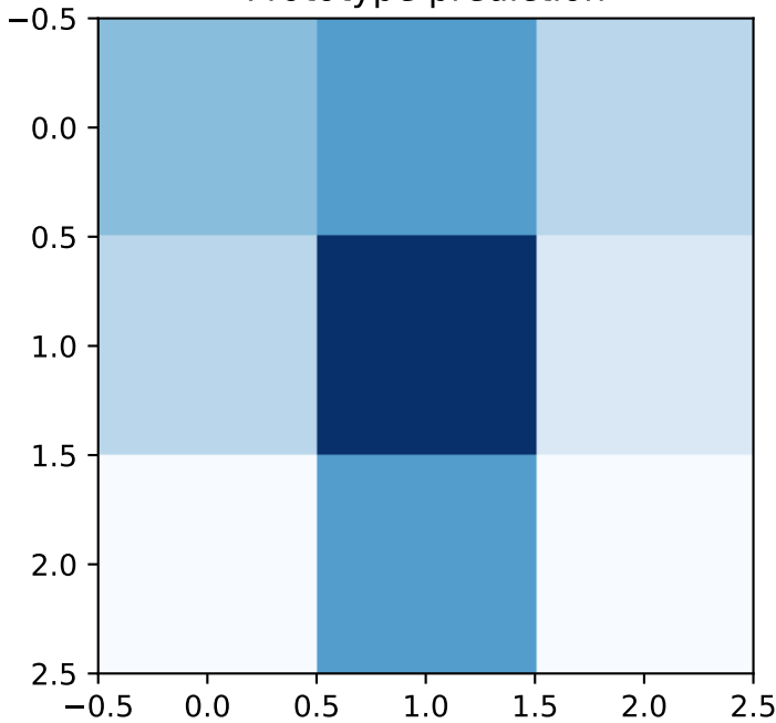
Prototype prediction
