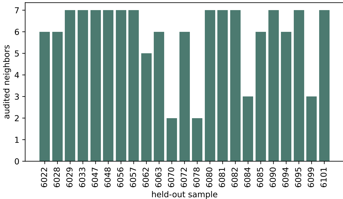
KNN neighbor audit
