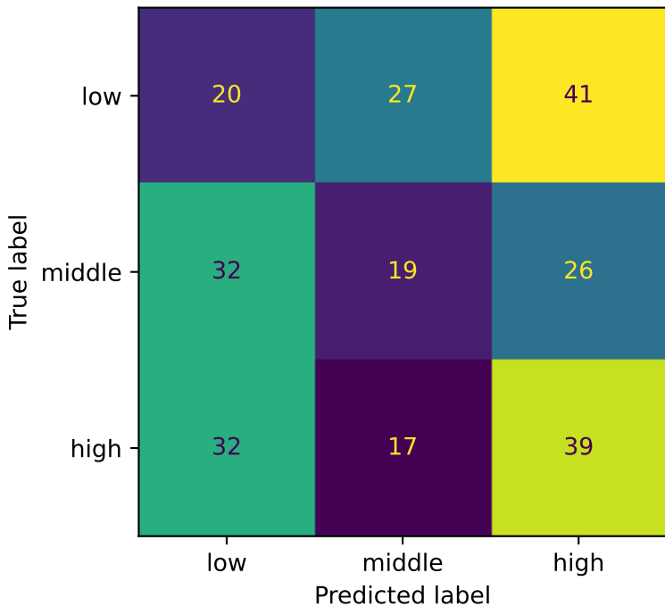
Low/middle/high confusion
