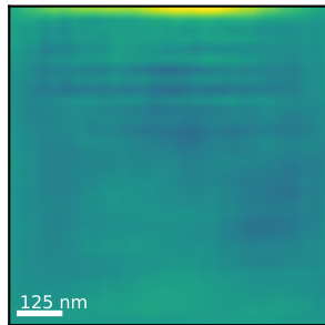
R_q=1.5 nm
