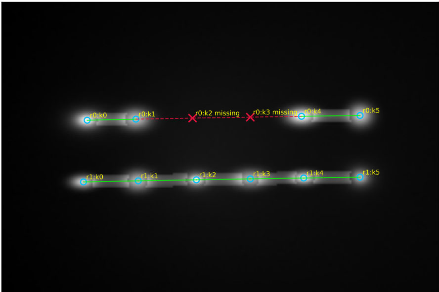
challenge_nearby_rows
