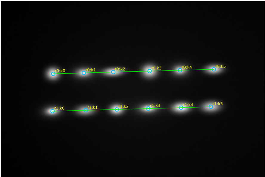
challenge_missing_two_sites
