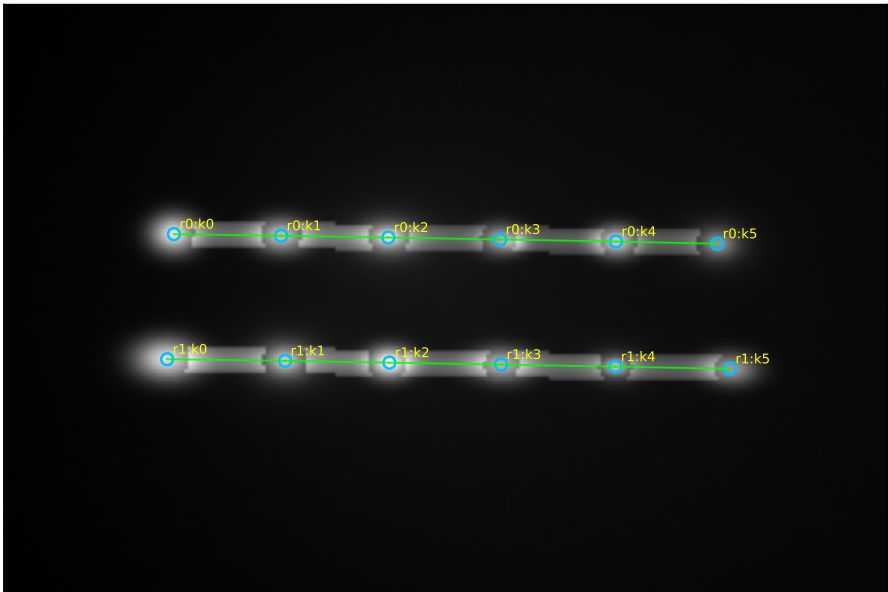
challenge_mild_curvature
