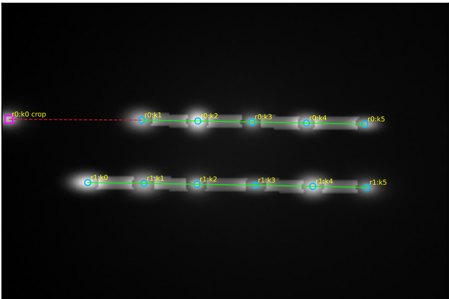
challenge_partial_crop_endpoint
