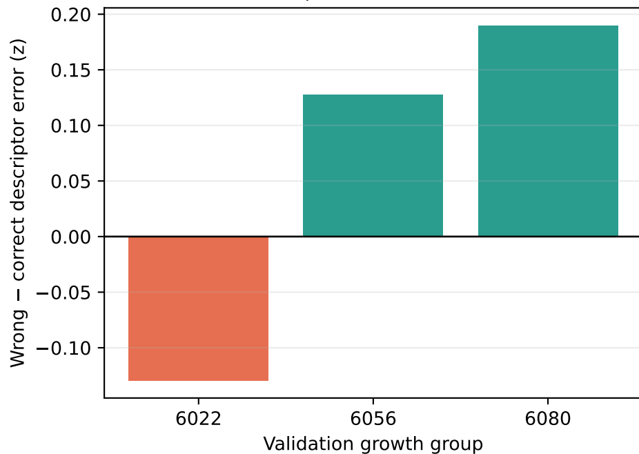
Spectral (RHEED)
