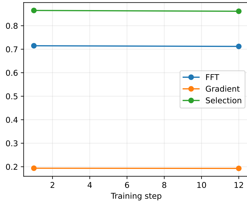
Validation-only early stopping
