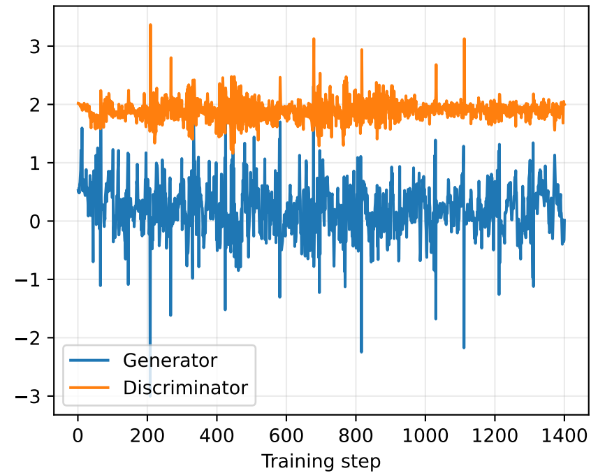
Adversarial losses
