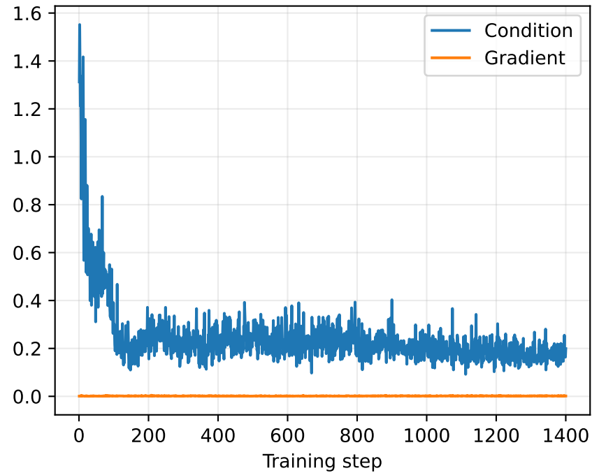
Scientific regularizers
