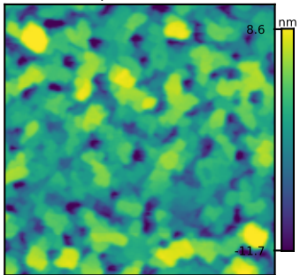
Retrieved Pred 4.27; GT T4 2.30 nm Rq = 4.27 nm
