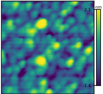
Ground truth 1 Rq = 0.74 nm
