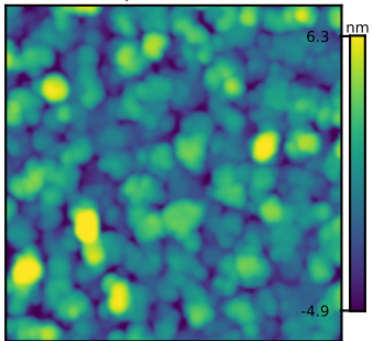
Ground truth 3 Rq = 2.29 nm
