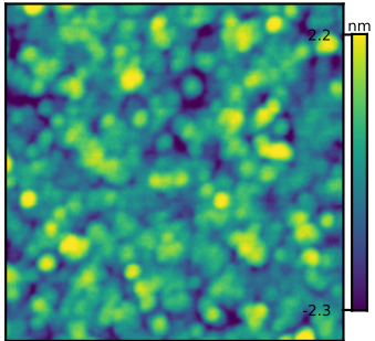
Ground truth 3 Rq = 0.92 nm
