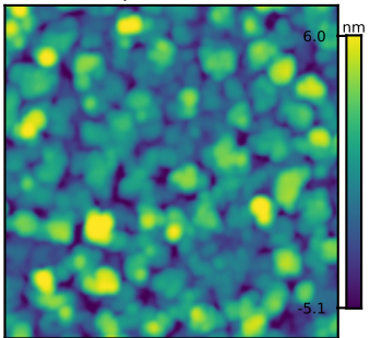
Ground truth 1 Rq = 2.40 nm
