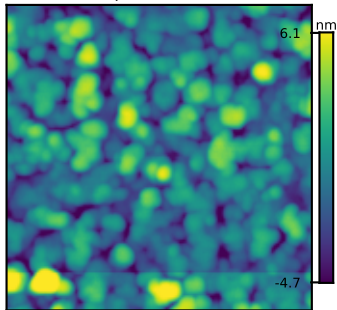
Ground truth 4 Rq = 2.25 nm
