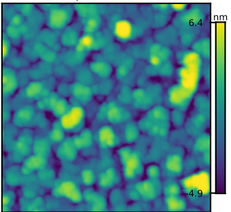
Ground truth 2 Rq = 2.36 nm
