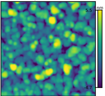
Ground truth 5 Rq = 2.15 nm
