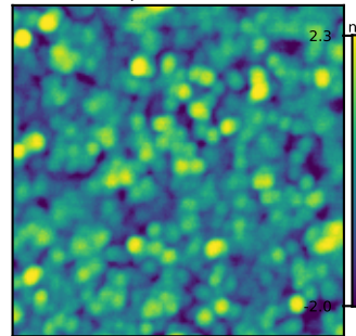
Ground truth 4 Rq = 0.88 nm
