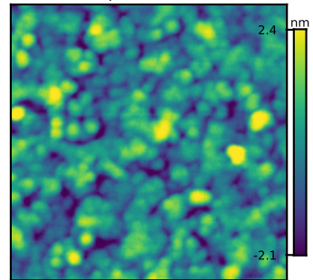
Ground truth 2 Rq = 0.93 nm
