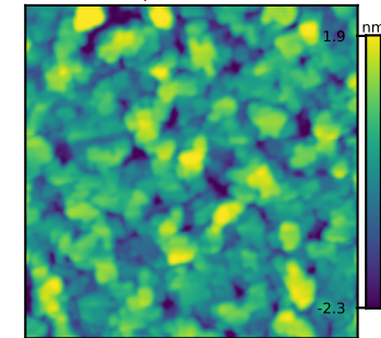
Retrieved Pred 0.88; GT T4 0.89 nm Rq = 0.88 nm
