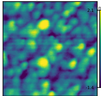
Ground truth 1 Rq = 0.74 nm
