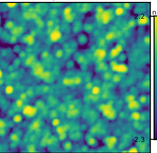
Ground truth 3 Rq = 0.92 nm
