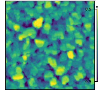
Retrieved Pred 3.78; GT T4 2.34 nm R_q = 3.78 nm
