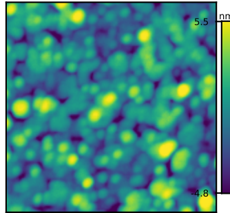
Ground truth 2 R_q = 2.16 nm
