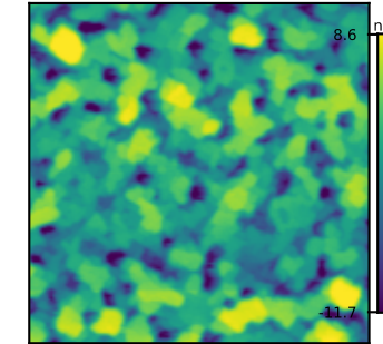
Retrieved Pred 4.27; GT T4 2.30 nm Rq = 4.27 nm
