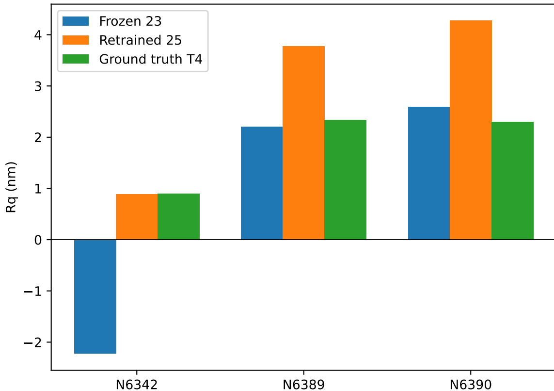
Frozen-model and retrained-model predictions
