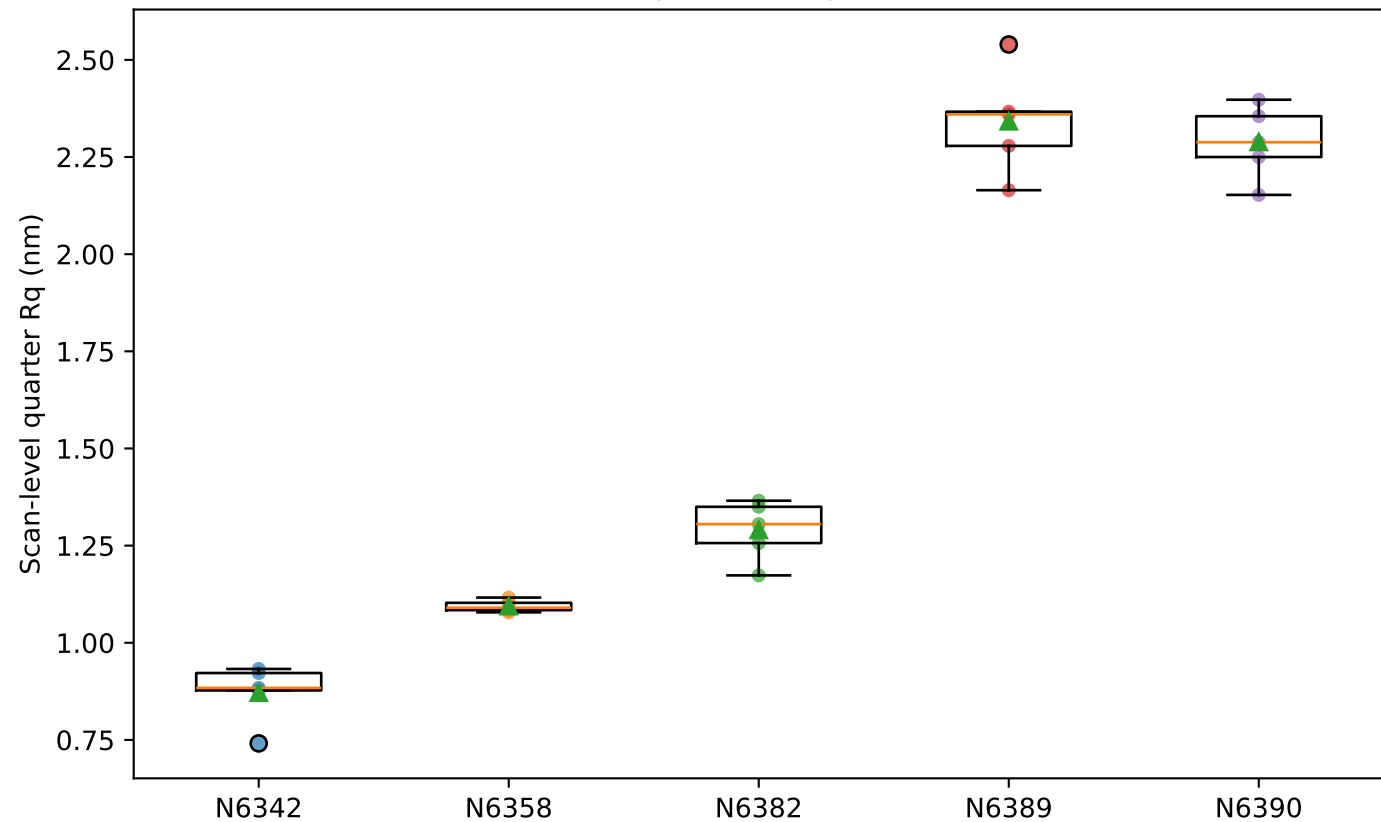
Within-sample AFM Rq distributions
