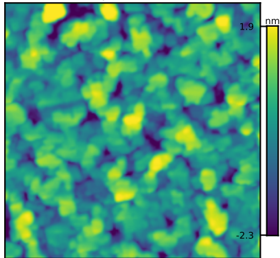
N6342 retrieved source 6048 R_q = 0.88 nm
