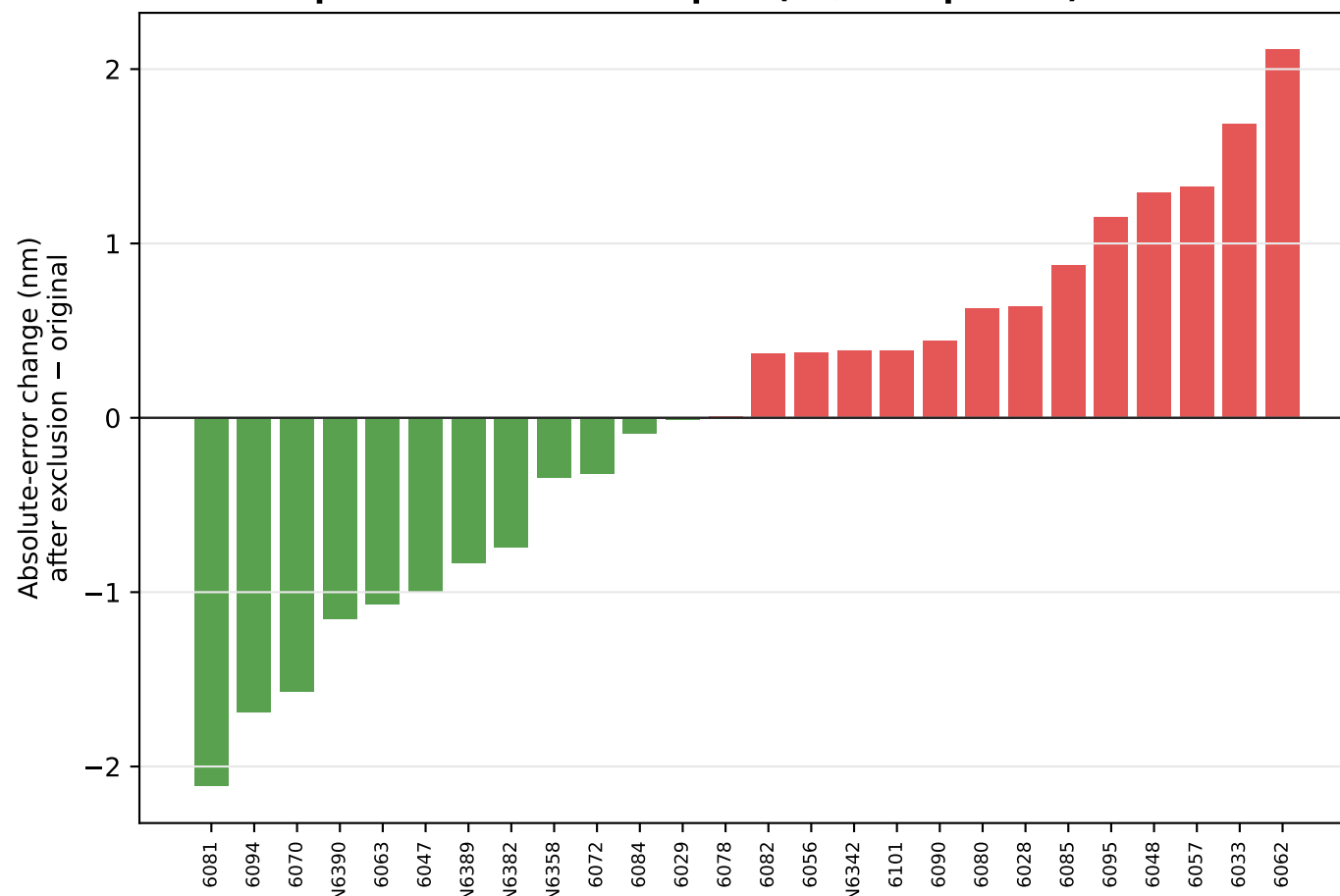
D LOO impact on retained samples (12/26 improved)
