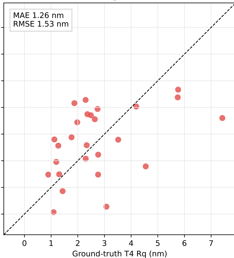
After excluding 6022 and 6099
