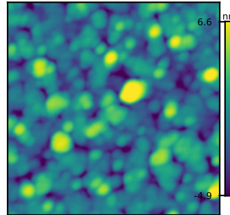
Ground truth 5 R_q = 2.28 nm
