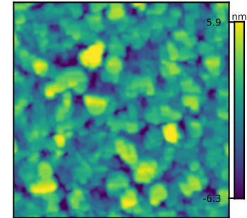
Retrieved Pred 2.52; GT T4 2.34 nm R_q = 2.52 nm
