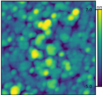
Ground truth 4 R_q = 2.37 nm
