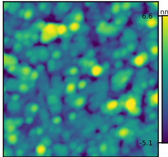
Ground truth 1 R_q = 2.36 nm
