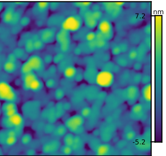
Ground truth 3 R_q = 2.54 nm
