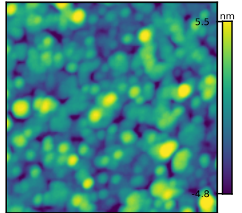
Ground truth 2 R_q = 2.16 nm
