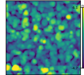
Ground truth 4 Rq = 2.25 nm
