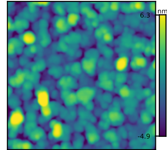
Ground truth 3 Rq = 2.29 nm
