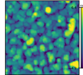
Ground truth 2 Rq = 2.36 nm
