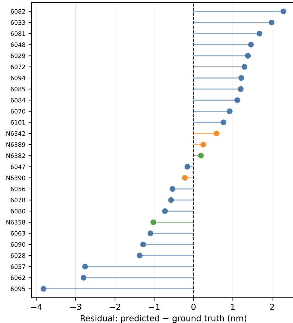
B Per-sample leave-one-out residuals
