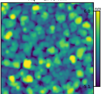
N6390 GT 1 Rq = 2.40 nm
