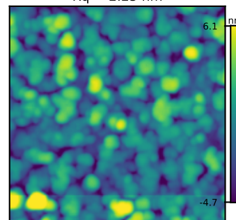
N6390 GT 4 Rq = 2.25 nm
