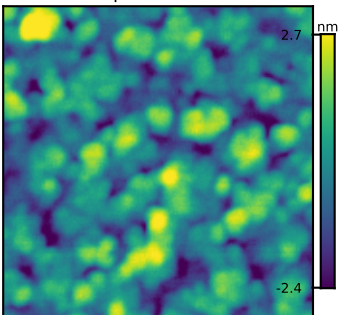
N6358 GT 1 Rq = 1.10 nm
