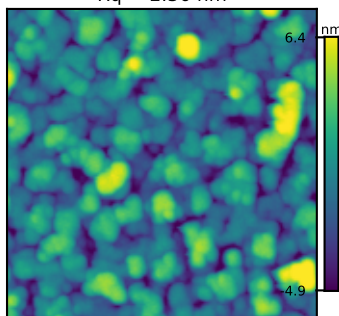
N6390 GT 2 Rq = 2.36 nm
