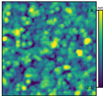
N6342 GT 2 Rq = 0.93 nm
