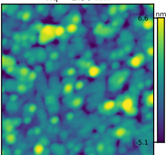
N6389 GT 1 Rq = 2.36 nm
