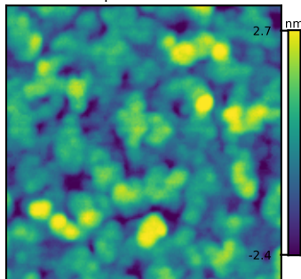
N6358 GT 2 Rq = 1.08 nm
