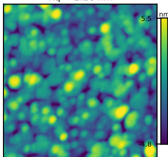
N6389 GT 2 Rq = 2.16 nm
