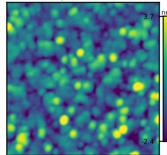
N6382 GT 4 Rq = 1.26 nm
