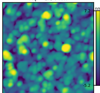
N6389 GT 3 Rq = 2.54 nm
