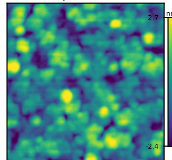
N6358 GT 4 Rq = 1.09 nm
