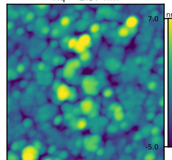
N6389 GT 4 Rq = 2.37 nm
