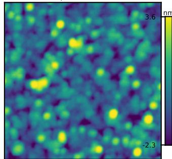
N6382 GT 3 Rq = 1.17 nm
