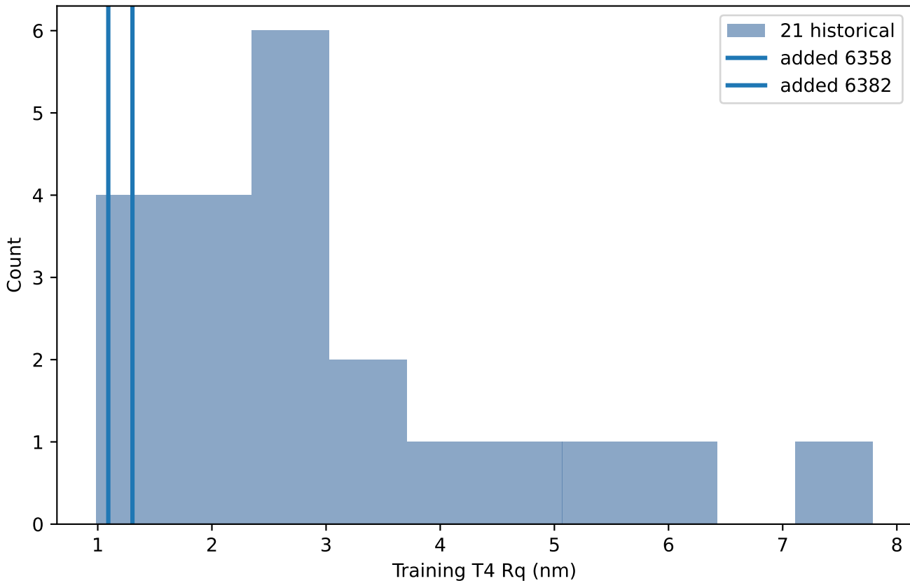
Training-target distribution after adding N6358 and N6382
