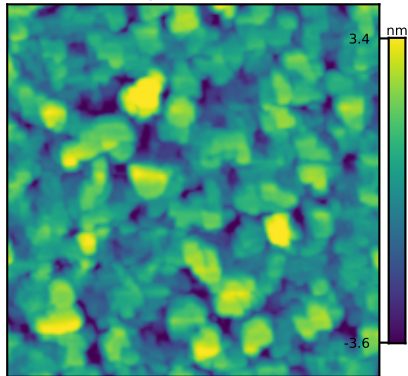
N6342 retrieved source 6028 R_q = 1.45 nm
