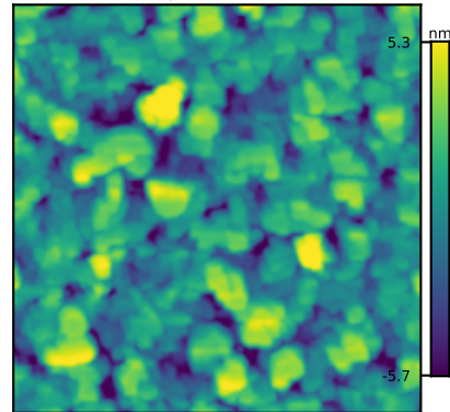
N6390 retrieved source 6028 R_q = 2.25 nm
