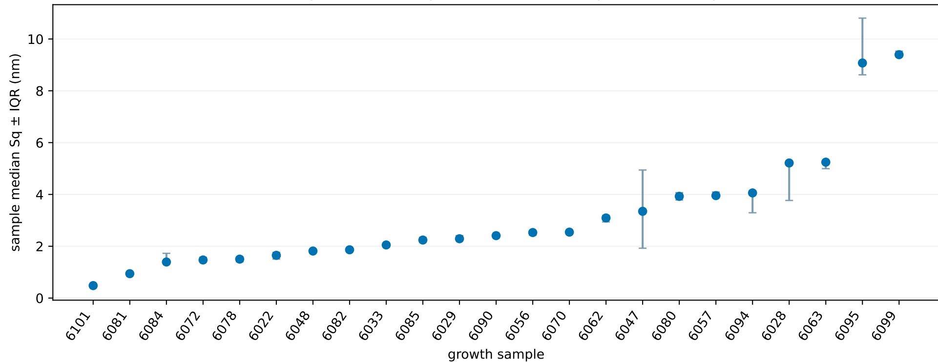
Corrected 23-growth AFM target distribution (deduplicated 1 × 1 μm scans)
