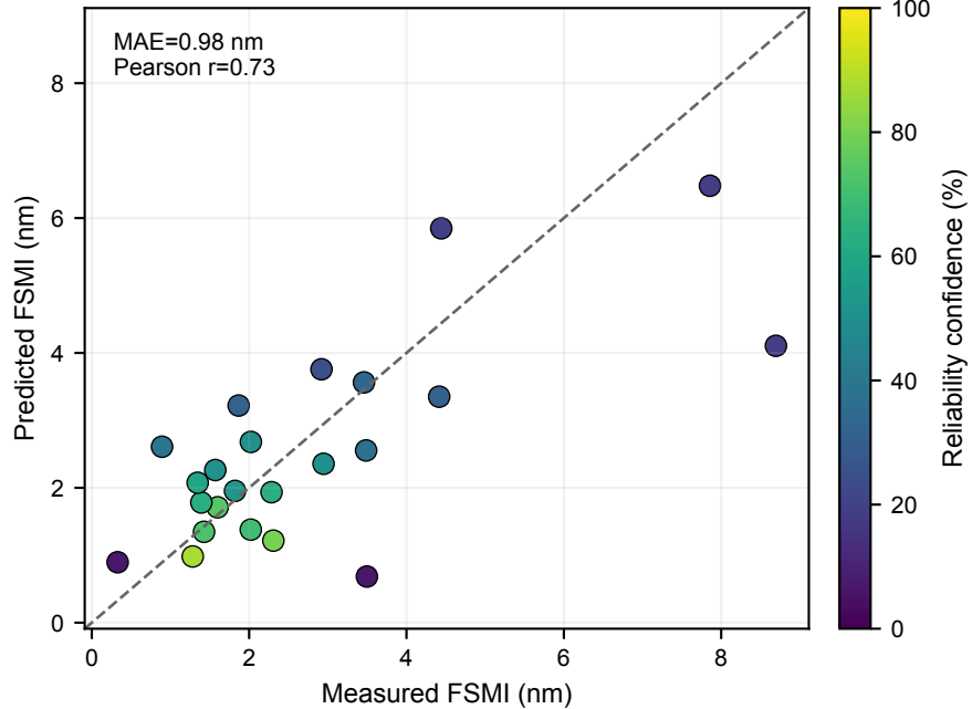
FSMI: strict 23-fold automatic-input LOO
