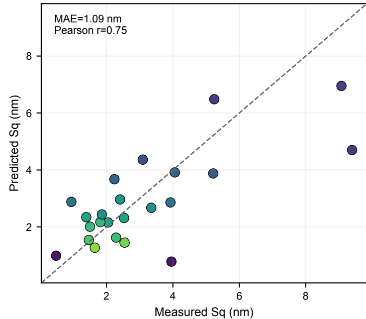
Sq: strict 23-fold automatic-input LOO
