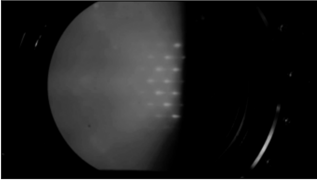
6082 RHEED key frame
