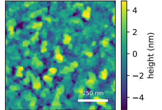
generated AFM predicted Sq=2.67 nm, FSMI=2.36 nm, C=50/100 measured AFM displayed scan Sq=2.00 nm sample median Sq=3.35 ± 3.02 nm (IQR)
