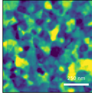
generated AFM predicted Sq=2.44 nm, FSMI=2.26 nm, C=50/100 measured AFM displayed scan Sq=1.86 nm sample median Sq=1.86 ± 0.12 nm (IQR)
