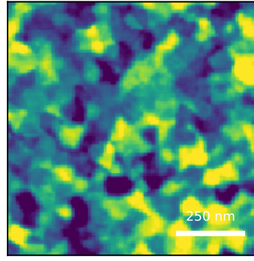
generated AFM predicted Sq=0.99 nm, FSMI=0.90 nm, C=7/100 measured AFM displayed scan Sq=0.57 nm sample median Sq=0.48 ± 0.09 nm (IQR)
