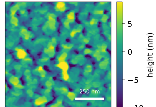
generated AFM predicted Sq=0.78 nm, FSMI=0.68 nm, C=7/100 measured AFM displayed scan Sq=3.95 nm sample median Sq=3.95 ± 0.19 nm (IQR)
