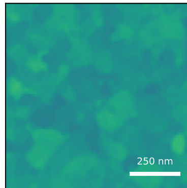
generated AFM predicted Sq=0.78 nm, FSMI=0.68 nm, C=7/100 measured AFM displayed scan Sq=3.95 nm sample median Sq=3.95 ± 0.19 nm (IQR)
