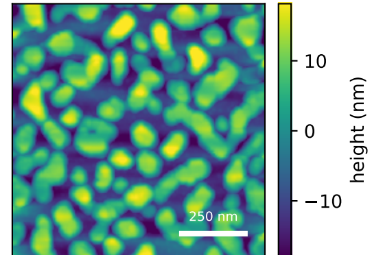
generated AFM predicted Sq=4.70 nm, FSMI=4.11 nm, C=18/100 measured AFM displayed scan Sq=9.39 nm sample median Sq=9.39 ± 0.21 nm (IQR)
