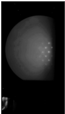
6099 RHEED key frame
