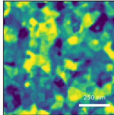
generated AFM predicted Sq=2.67 nm, FSMI=2.36 nm, C=50/100 measured AFM displayed scan Sq=2.00 nm sample median Sq=3.35 ± 3.02 nm (IQR)
