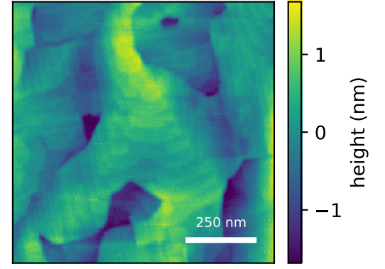
generated AFM predicted Sq=0.99 nm, FSMI=0.90 nm, C=7/100 measured AFM displayed scan Sq=0.57 nm sample median Sq=0.48 ± 0.09 nm (IQR)
