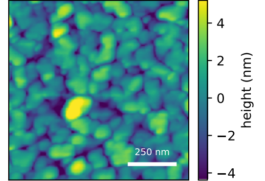
generated AFM predicted Sq=2.44 nm, FSMI=2.26 nm, C=50/100 measured AFM displayed scan Sq=1.86 nm sample median Sq=1.86 ± 0.12 nm (IQR)
