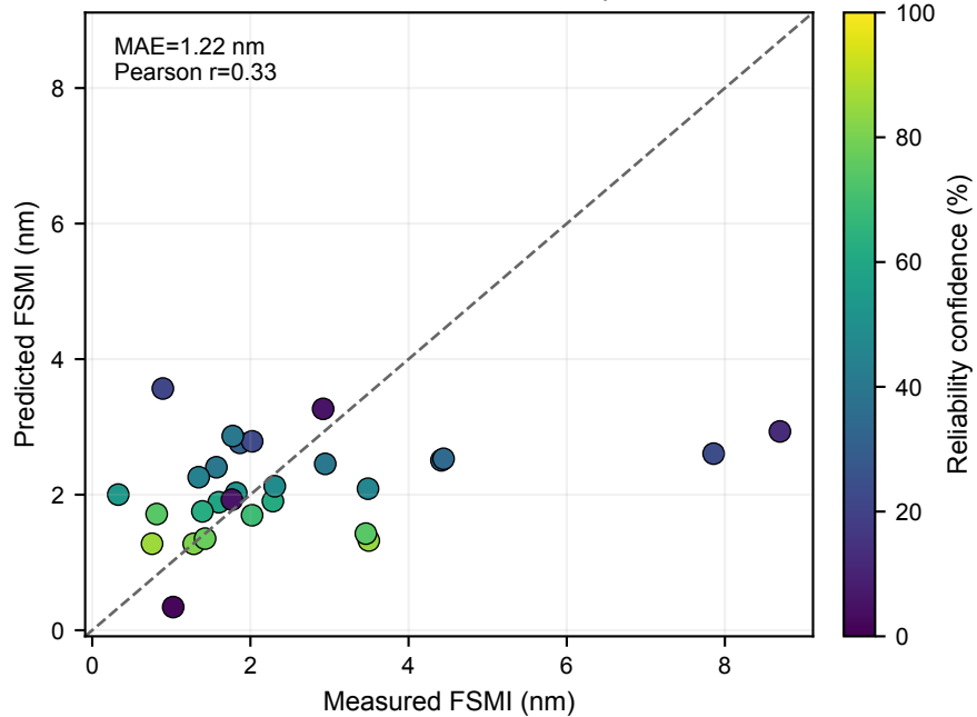
FSMI: strict 28-fold automatic-input LOO
