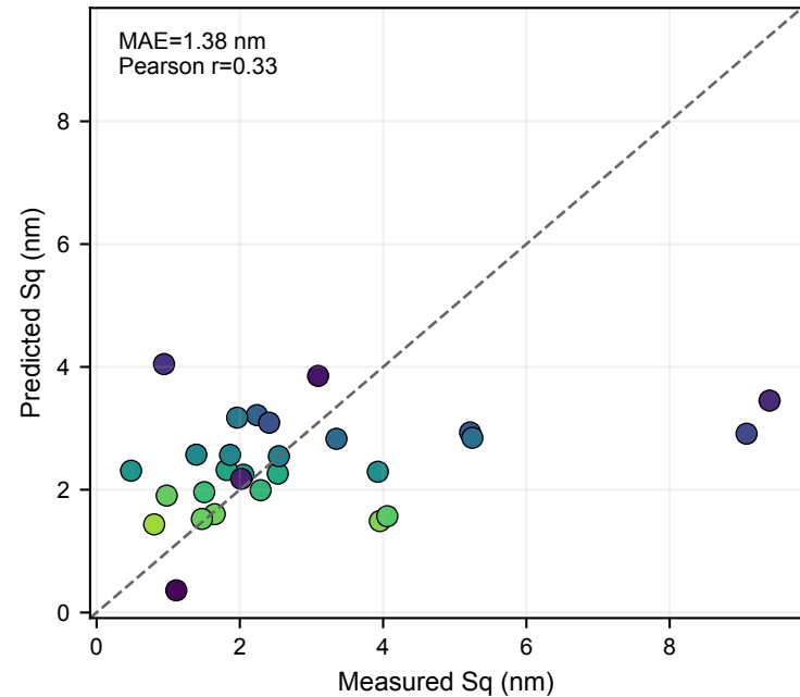
Sq: strict 28-fold automatic-input LOO
