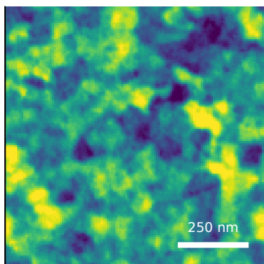
M10 baseline predicted S_q=1.69 nm
