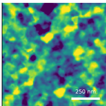
M10 baseline predicted S_q=3.86 nm
