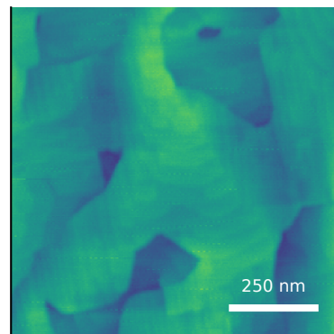
measured AFM displayed scan S_q=1.56 nm sample median S_q=1.50 \pm 0.18 nm (IQR)
