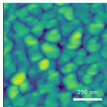
measured AFM displayed scan S_q=2.00 nm sample median S_q=3.35 \pm 3.02 nm (IQR)
