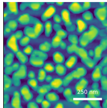
measured AFM displayed scan S_q=9.39 nm sample median S_q=9.39 \pm 0.21 nm (IQR)
