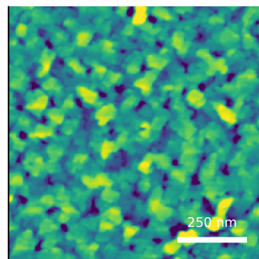
measured AFM displayed scan S_q=2.18 nm sample median S_q=2.24 \pm 0.18 nm (IQR)
