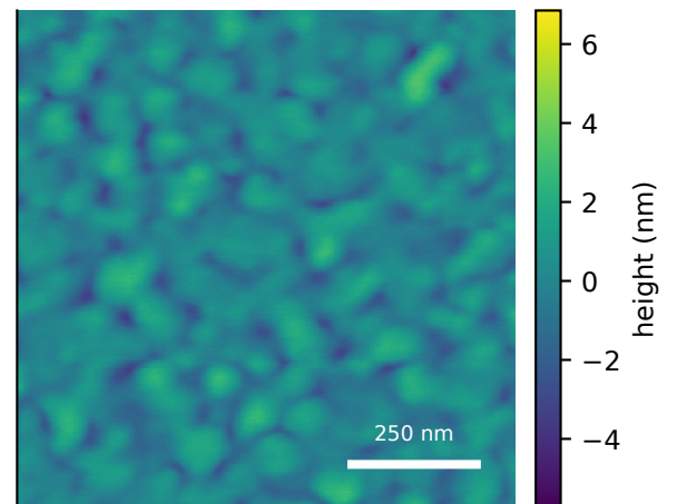
measured AFM displayed scan Sq=0.94 nm sample median Sq=0.94 ± 0.03 nm (IQR)
