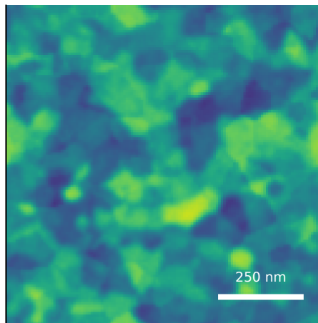
generated AFM predicted Sq=0.79 nm; FSMI=0.70 nm C=76/100
