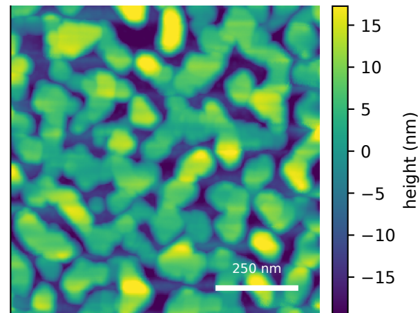
measured AFM displayed scan Sq=9.39 nm sample median Sq=9.39 ± 0.21 nm (IQR)
