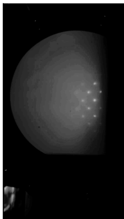
6099 RHEED key frame
