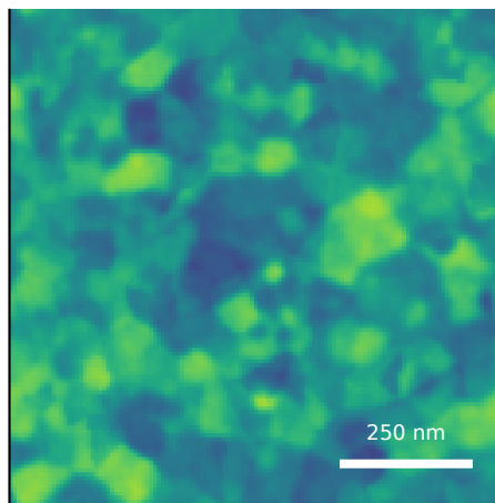
generated AFM predicted Sq=5.24 nm; FSMI=4.45 nm C=10/100
