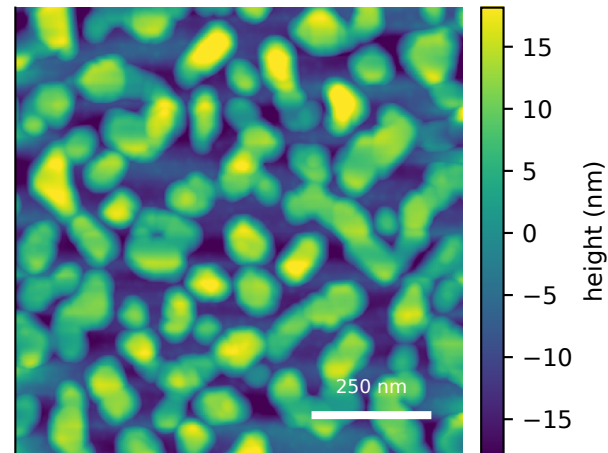
measured AFM displayed scan Sq=3.95 nm sample median Sq=3.95 ± 0.19 nm (IQR)
