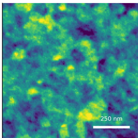
M10 dense-island spectral predicted Sq=1.69 nm
