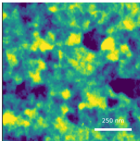
M10 dense-island spectral predicted Sq=1.84 nm
