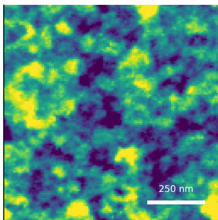
M10 dense-island spectral predicted Sq=0.62 nm
