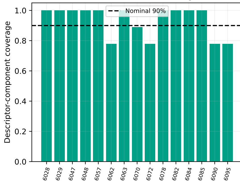
Strict cross-fitted coverage
