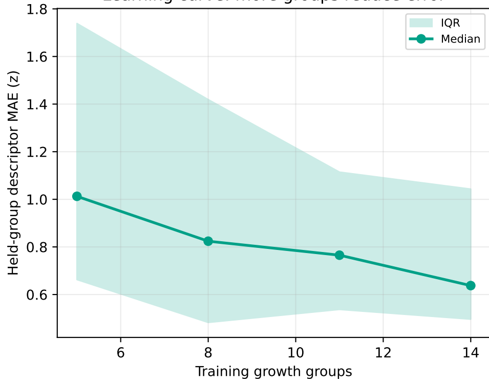
Learning curve: more groups reduce error
