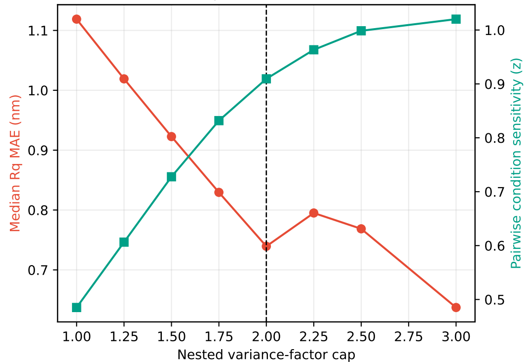
Sensitivity-error Pareto ablation
