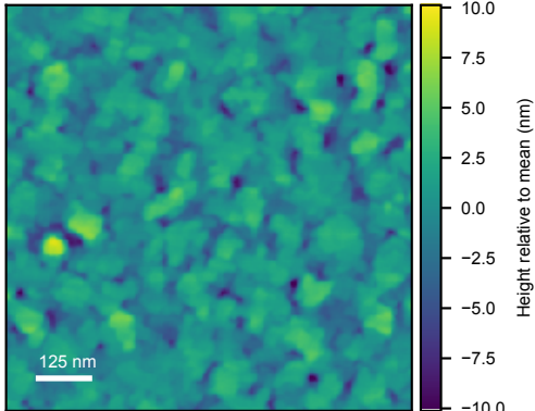
Retrieved real AFM exemplar source=6078 Rq=2.04 nm
