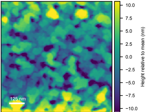
Ground-truth AFM Rq=5.87 nm Ra=4.63 nm
