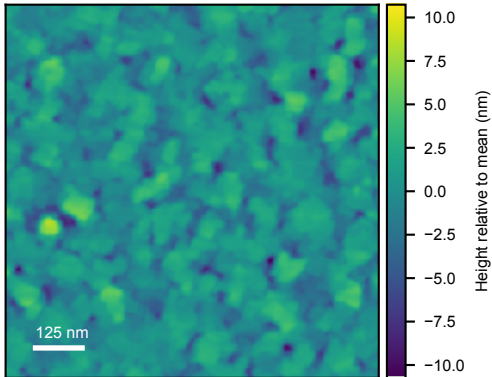
Retrieved real AFM exemplar source=6090 Rq=4.71 nm
