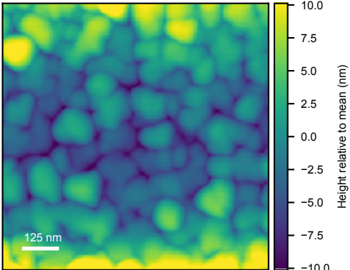
Ground-truth AFM Rq=5.34 nm Ra=4.14 nm
