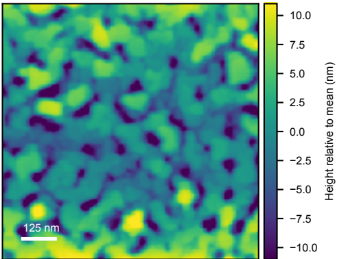
Ground-truth AFM Rq=4.69 nm Ra=3.77 nm
