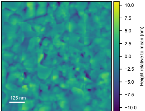
Retrieval-augmented representative AFM Rq=4.71 nm
