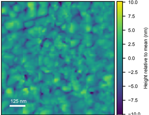
Retrieval-augmented representative AFM Rq=2.04 nm
