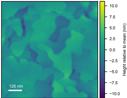
Retrieved real AFM exemplar source=6078 Rq=2.21 nm
