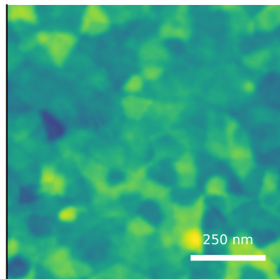
generated AFM Rq=2.51 nm, FSMI=2.05 nm, C=50/100
