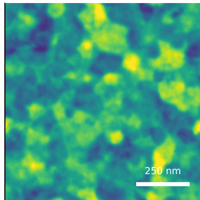
generated AFM Rq=3.63 nm, FSMI=3.22 nm, C=100/100
