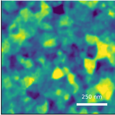
generated AFM Rq=2.70 nm, FSMI=1.95 nm, C=88/100
