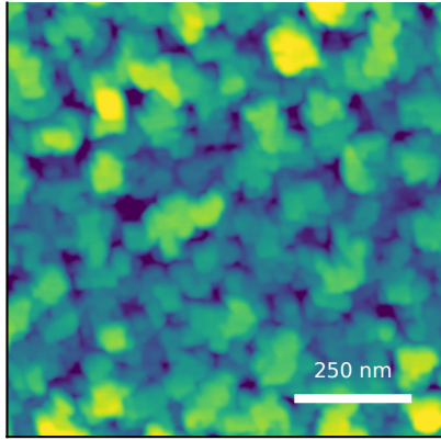
measured AFM Rq=3.05 nm, FSMI=2.62 nm
