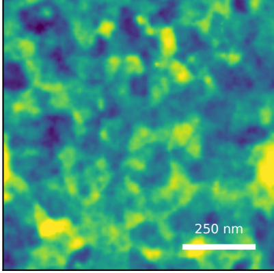
generated AFM Rq=2.95 nm, FSMI=2.30 nm, C=81/100
