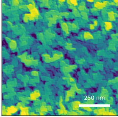
measured AFM Rq=3.07 nm, FSMI=2.95 nm
