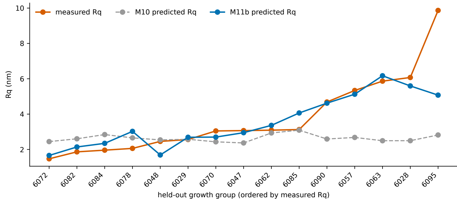
Dynamic-range recovery: the new amplitude head no longer collapses all predictions near 3 nm
